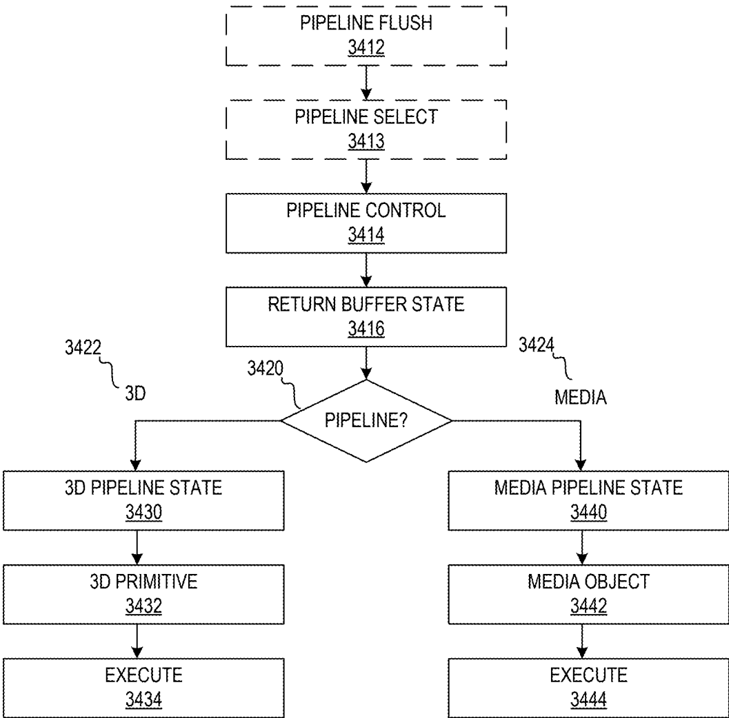
FIG. 34B GRAPHICS PROCESSOR COMMAND SEQUENCE 3410
