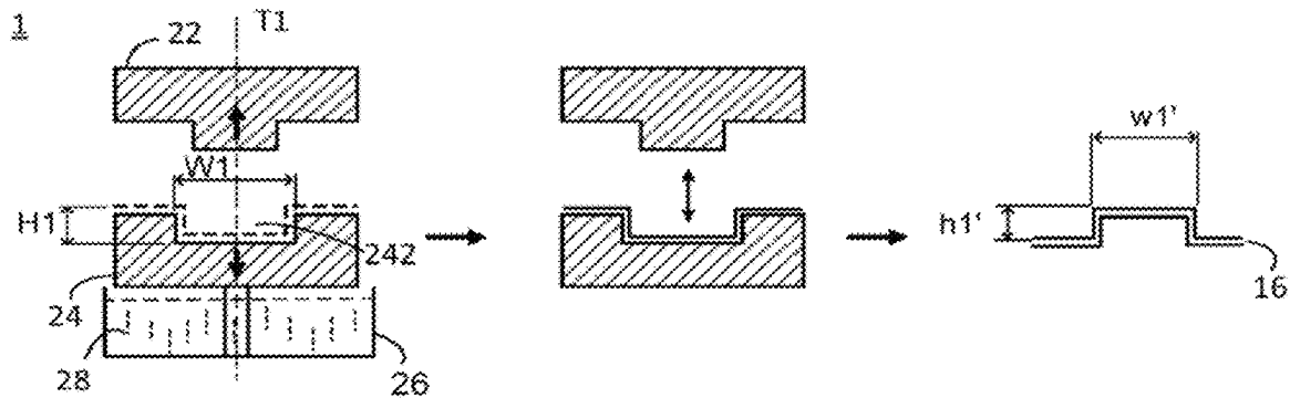
Fig. 1 (Prior Art)
