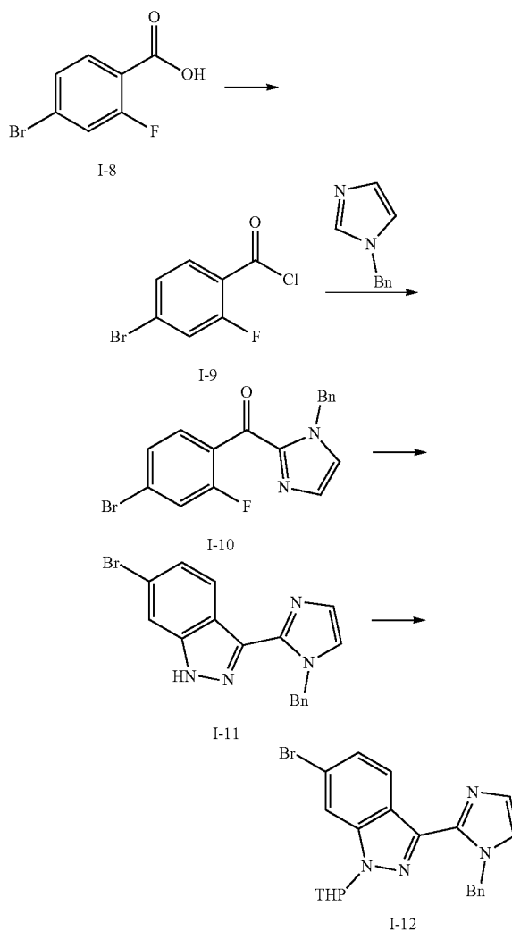
(a) 4-bromo-2-fluorobenzoyl chloride (I-9)
