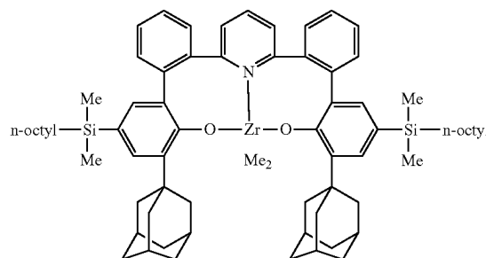
Complex 11
