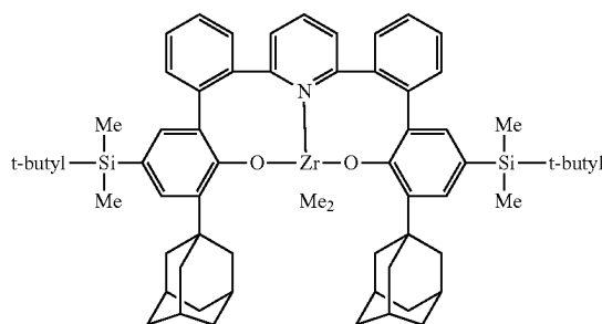
Complex 9
