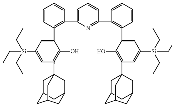
2',2'''-(pyridine-2,6-diyl)bis(3-(1-adamantany)-5-(triethylsilyl)-[1,1'-biphenyl]-2-ol)
