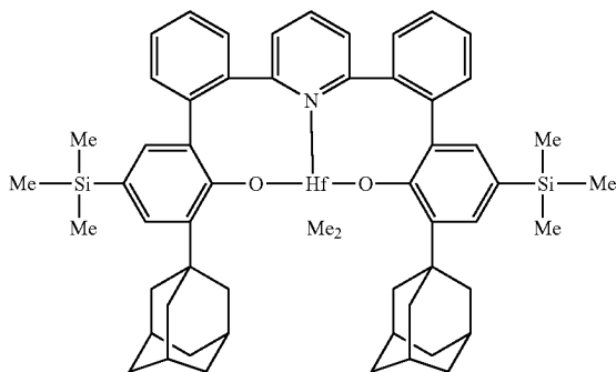
Complex 3
