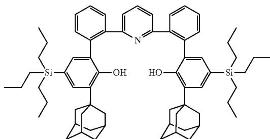
2',2'''-(pyridine-2,6-diyl)bis(3-(1-adamantyl)-5-(tripropylsilyl)-[1,1'-biphenyl]-2-ol)
