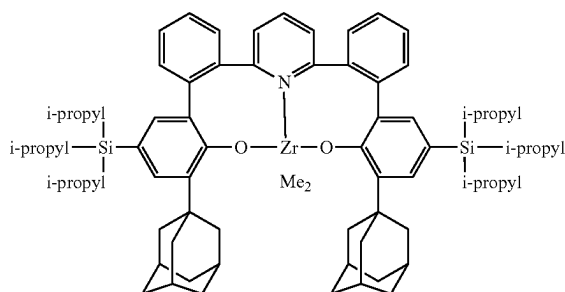
Complex 7
