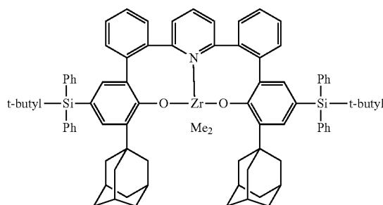
Complex 8
