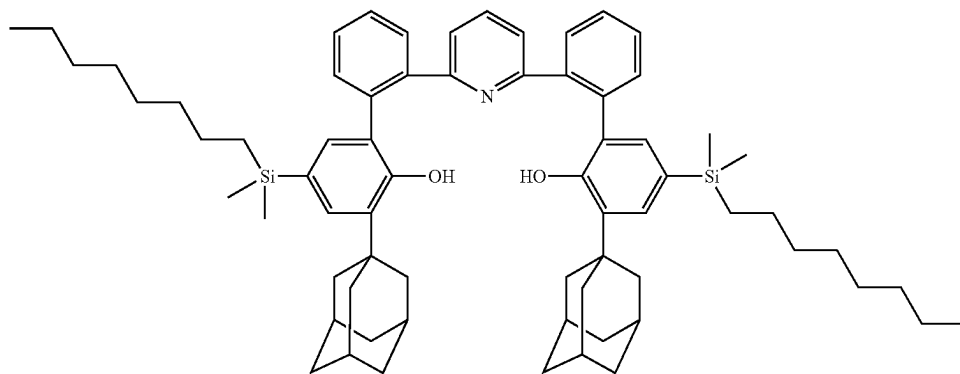
2',2'''-(pyridine-2,6-diyl)bis(3-(1-adamantyl)-5-(octyldimethylsilyl)-[1,1'-biphenyl]-2-ol)
