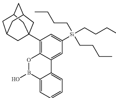
(4-(1-adamantyl)-6-hydroxybenzo[c][1,2]benzoxaborinin-2-yl)tributylsilane
