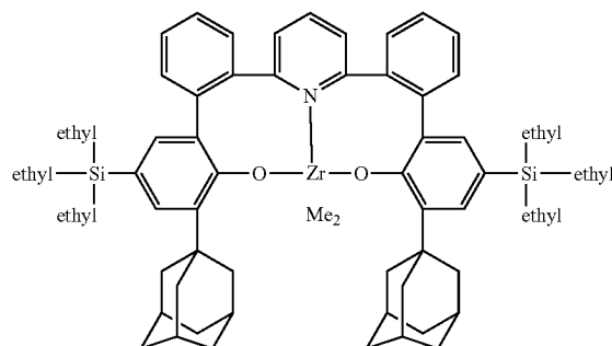
Complex 4
