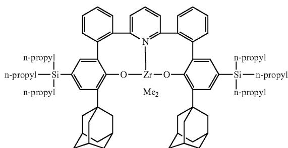
Complex 5
