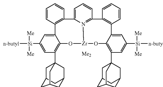
Complex 10
