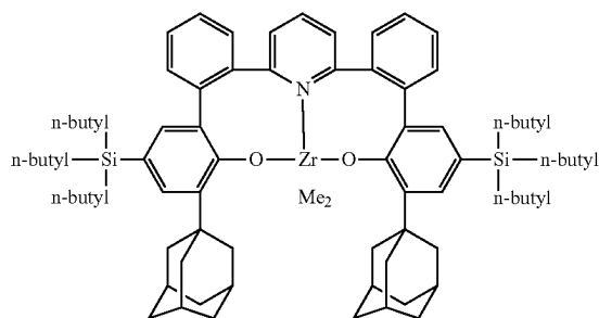
Complex 6
