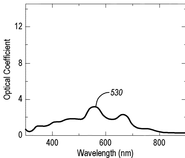
FIG. 5C (PRIOR ART)
