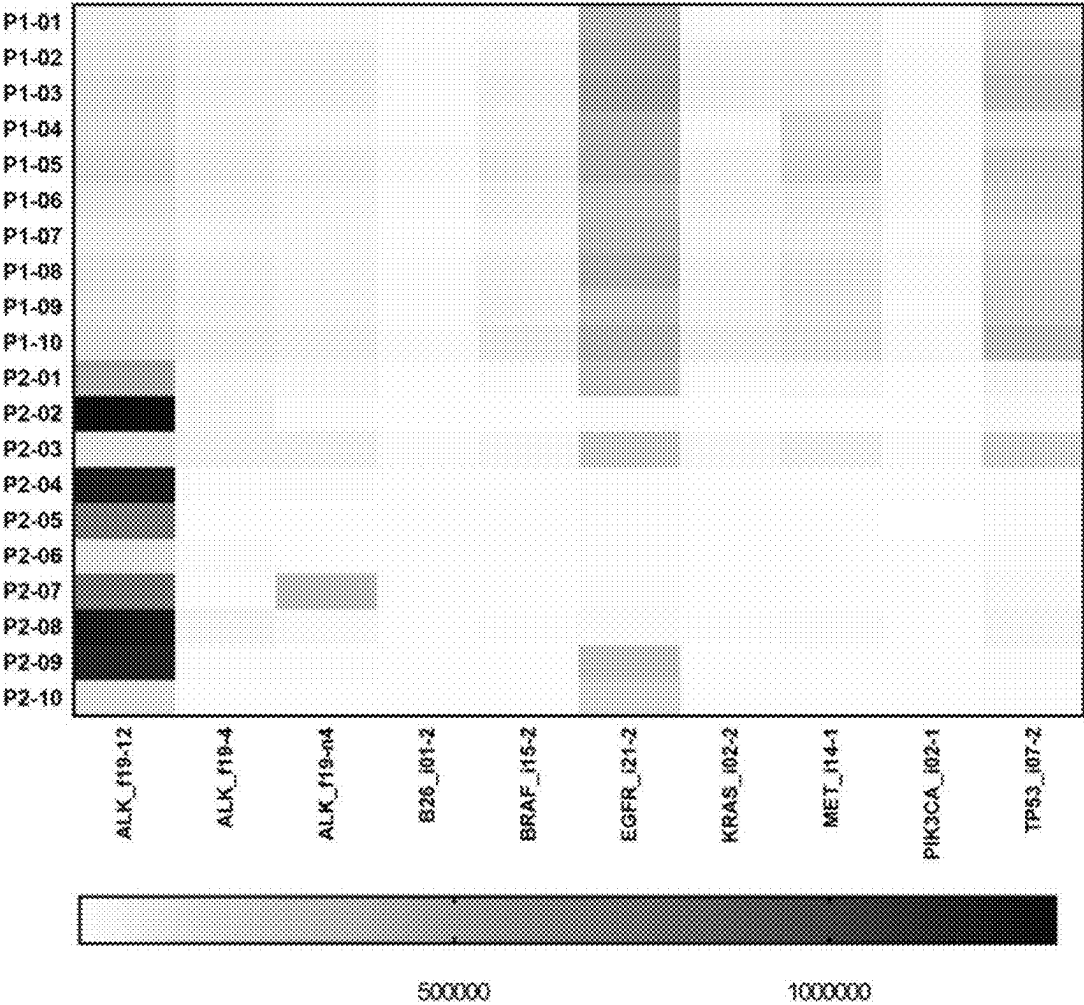
Reads obtained by amplification with different primers
