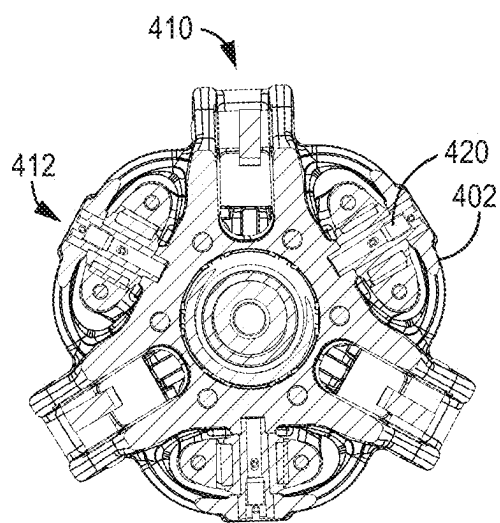
SECTION E-E FIG. 16I
