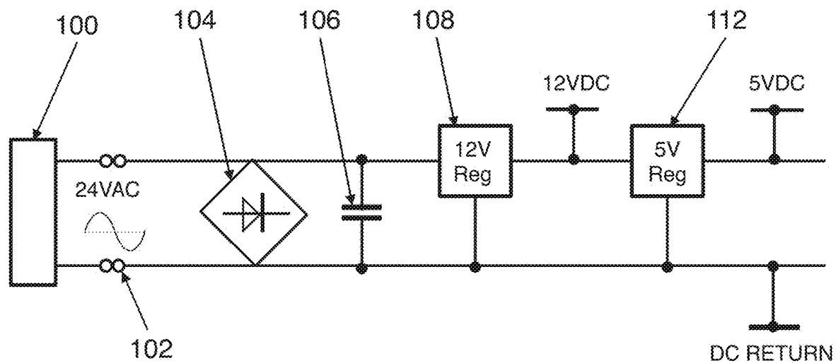
Fig. 5B Diagram of AC Power Scheme
