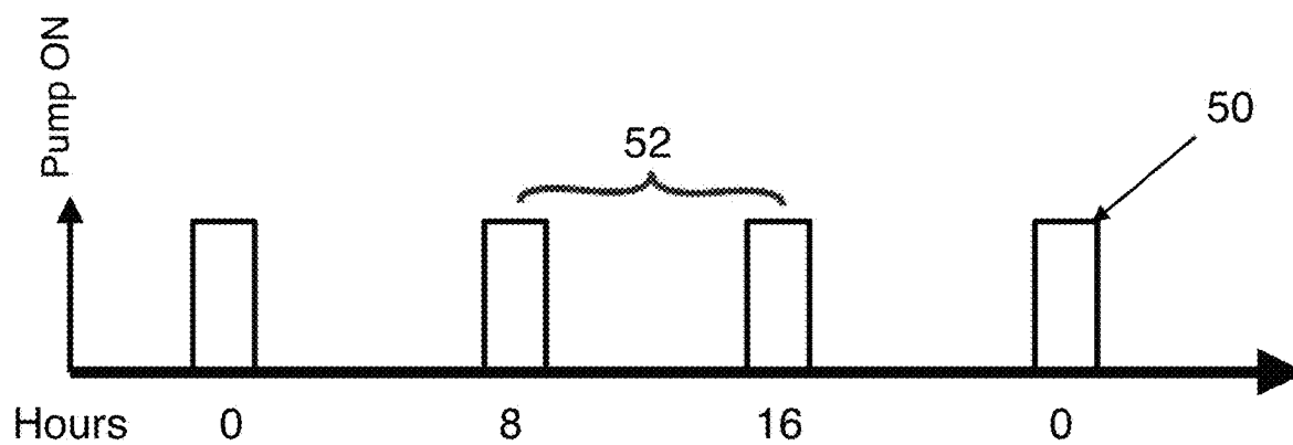
Fig. 4A Diagram of Dose and Interval at 25 C
