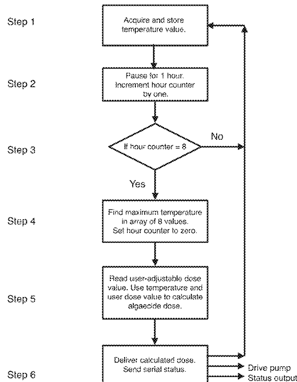
Flowchart of Algaecide Method
