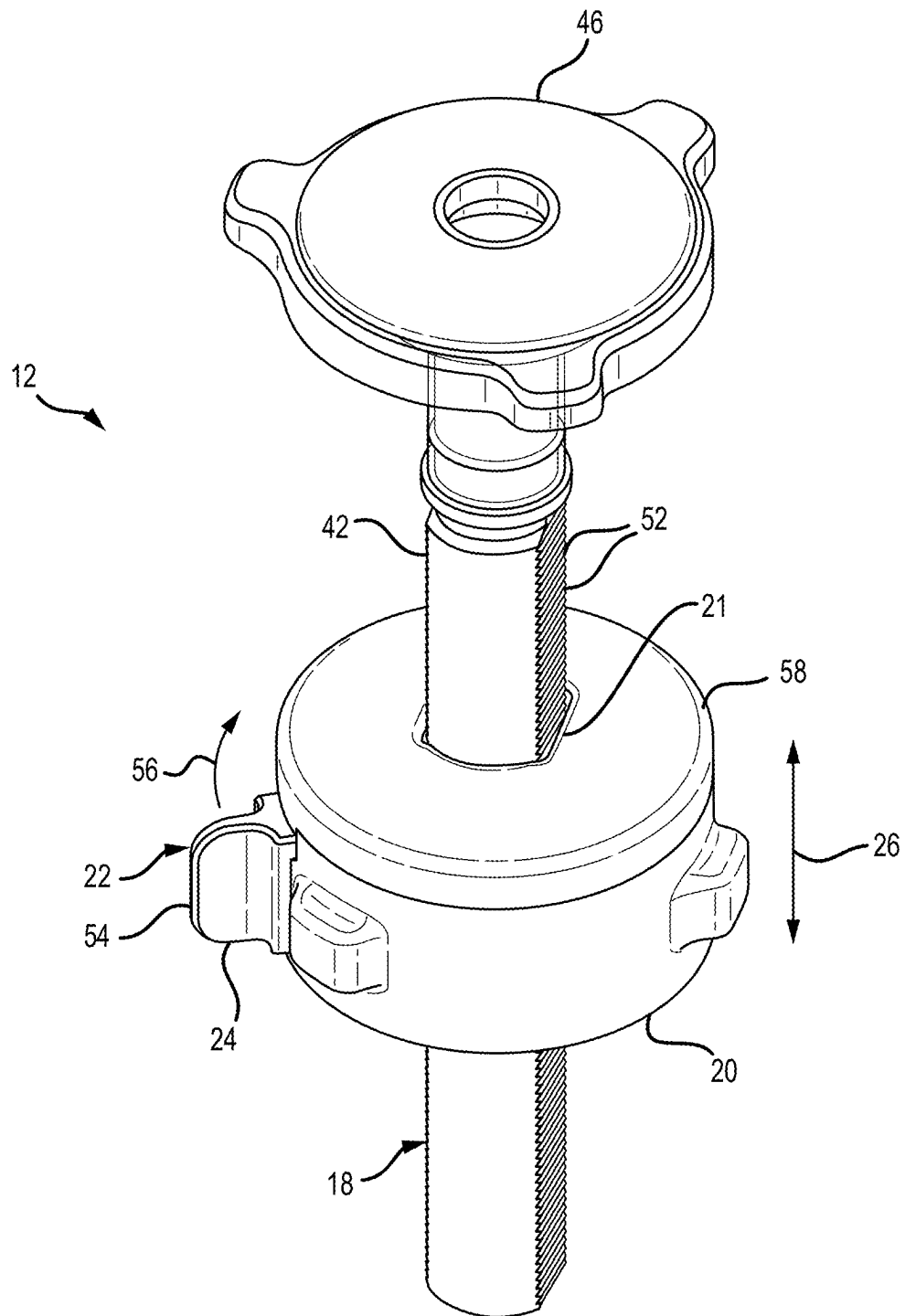
FIG. 6 (PRIOR ART)
