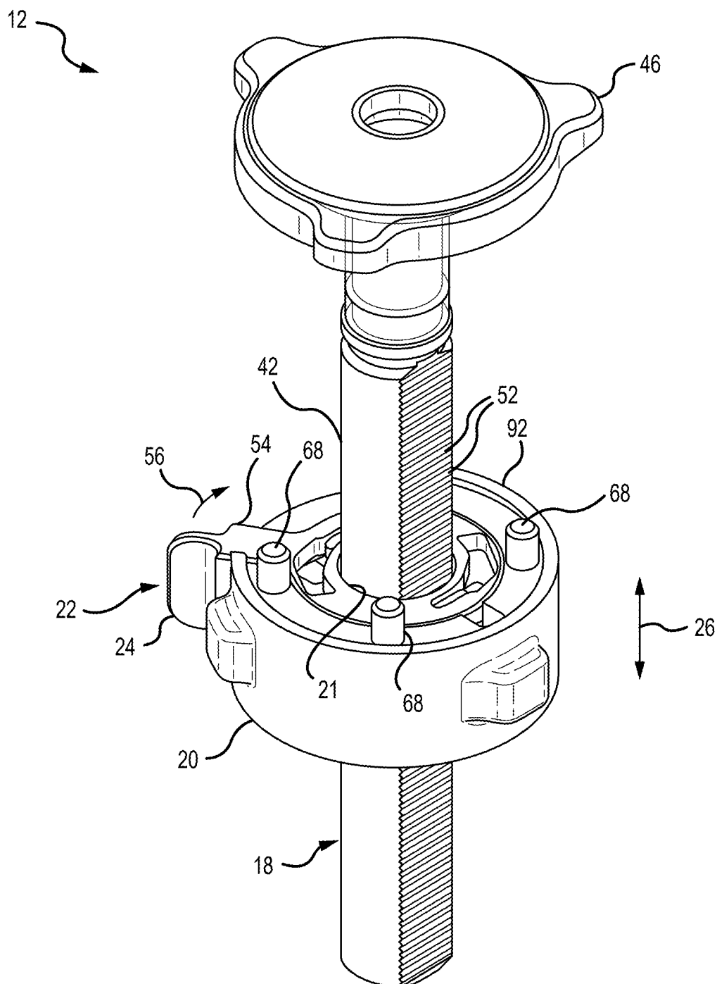
FIG. 7 (PRIOR ART)
