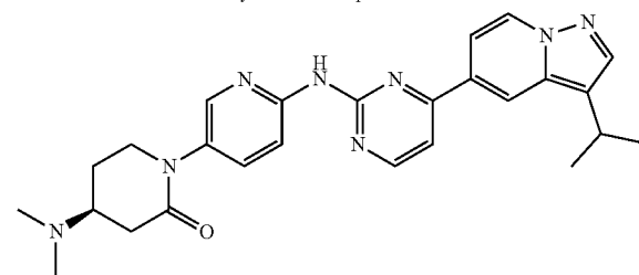
synthetic example 3
