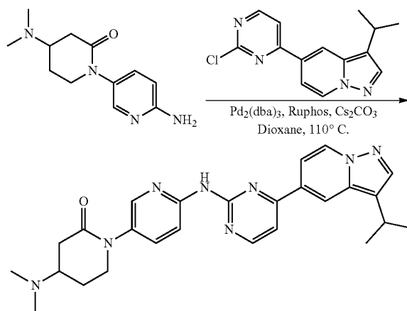
synthetic example 1
