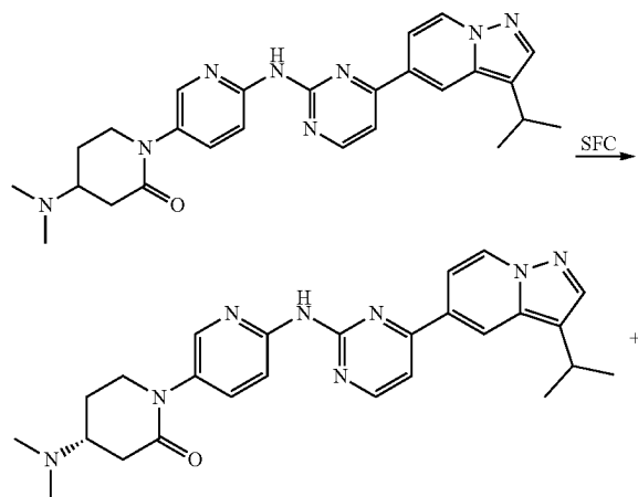
synthetic example 2
