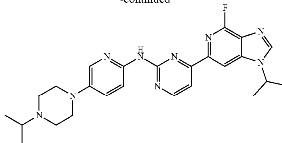
synthetic example 4
