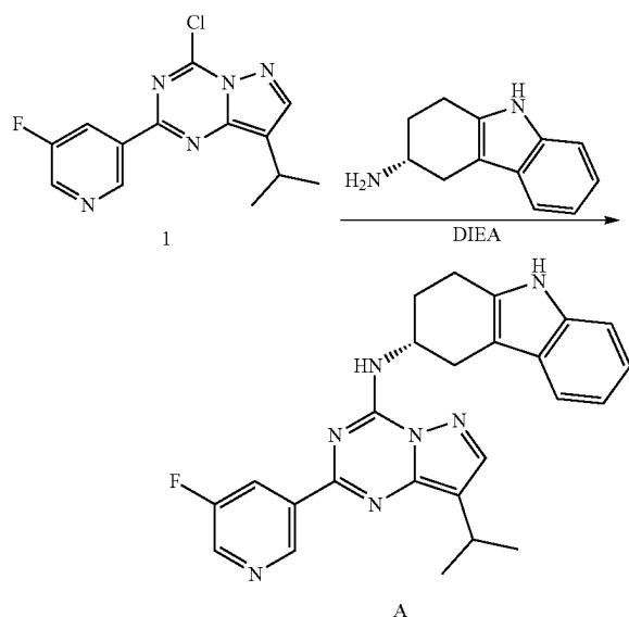
Scheme 1 - Synthesis of Compound A
