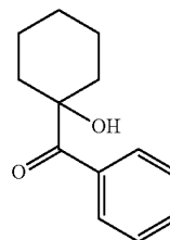
OMNIRAD 184
