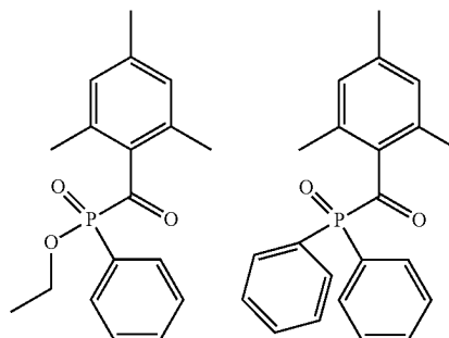
OMNIRAD TPO-L
