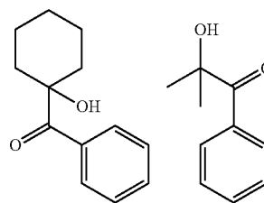
OMNIRAD 1000
