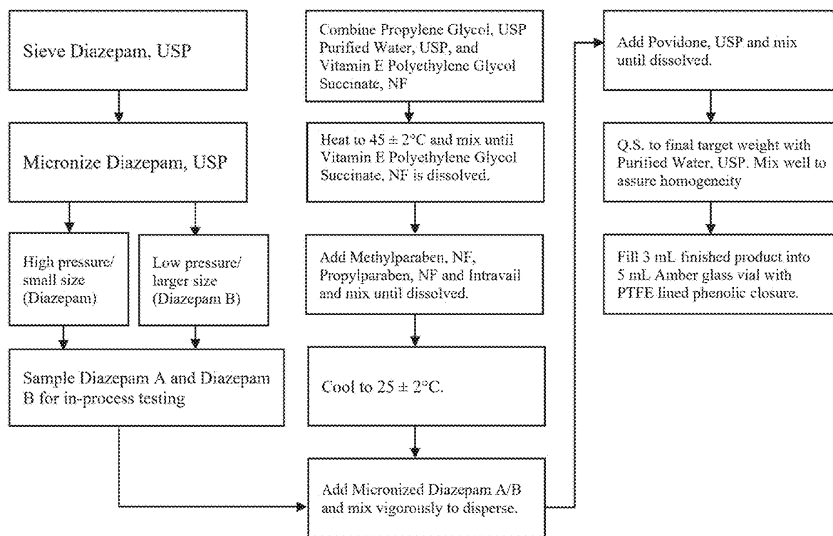
Flow Diagram for the Manufacture of NRL-1A
