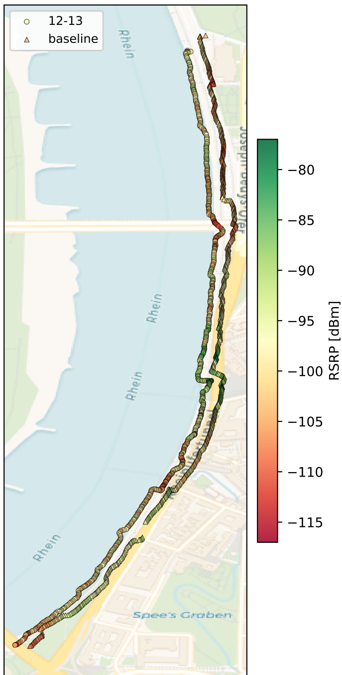
Telekom — RSRP: 12-13 (west, circles) vs. baseline (east, triangles)
