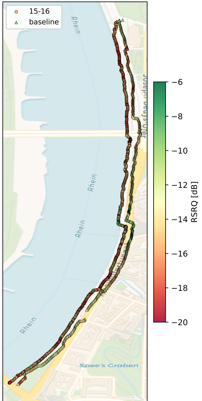
Telekom — RSRQ: 15-16 (west, circles) vs. baseline (east, triangles)
