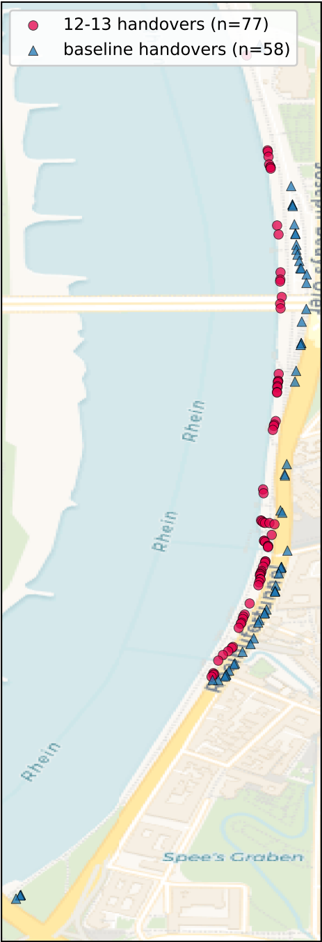
Telekom 12-13 — Handover locations: Event (west, circles) vs. baseline (east, triangles)
