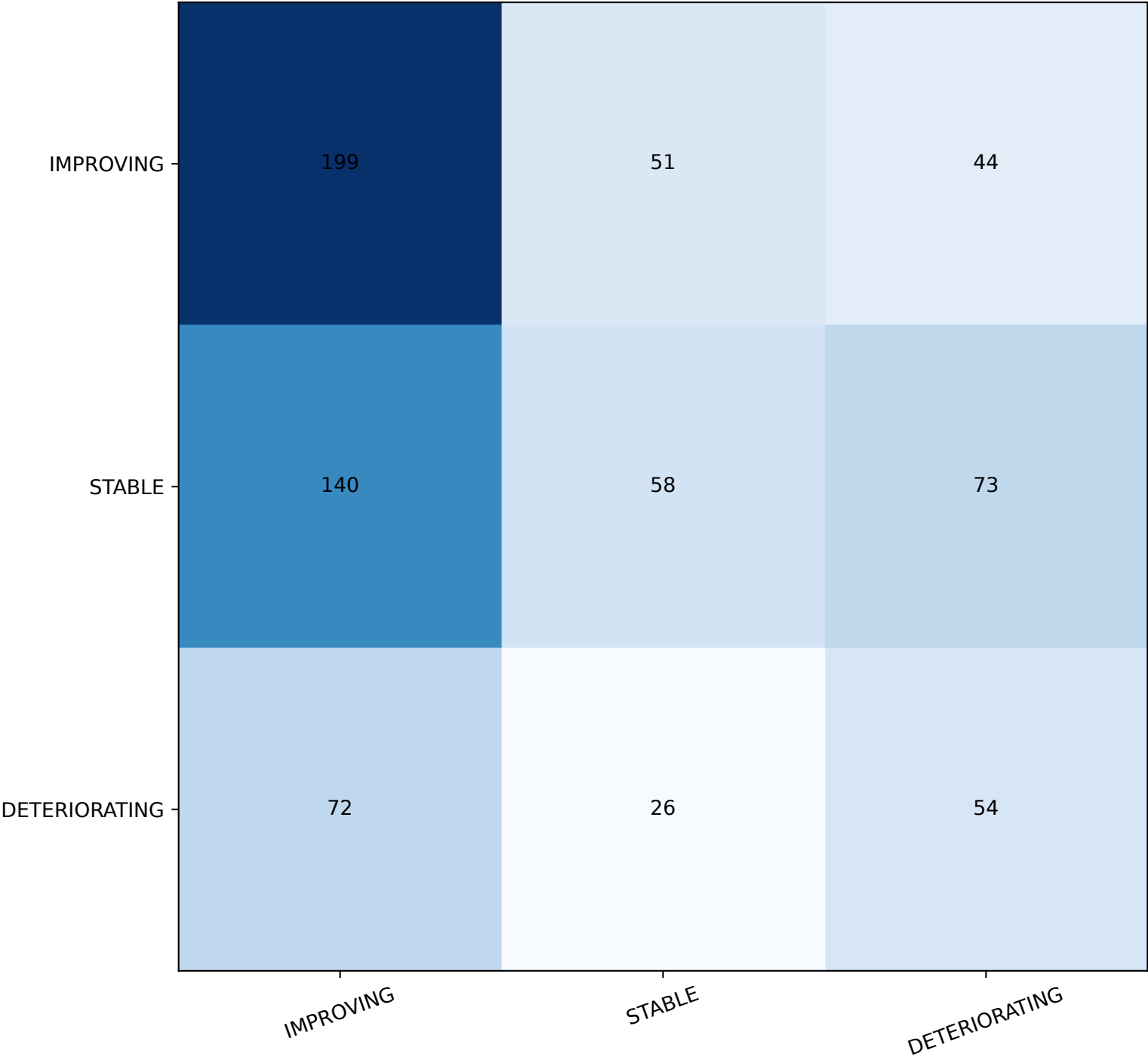
Frozen identification confusion matrix
