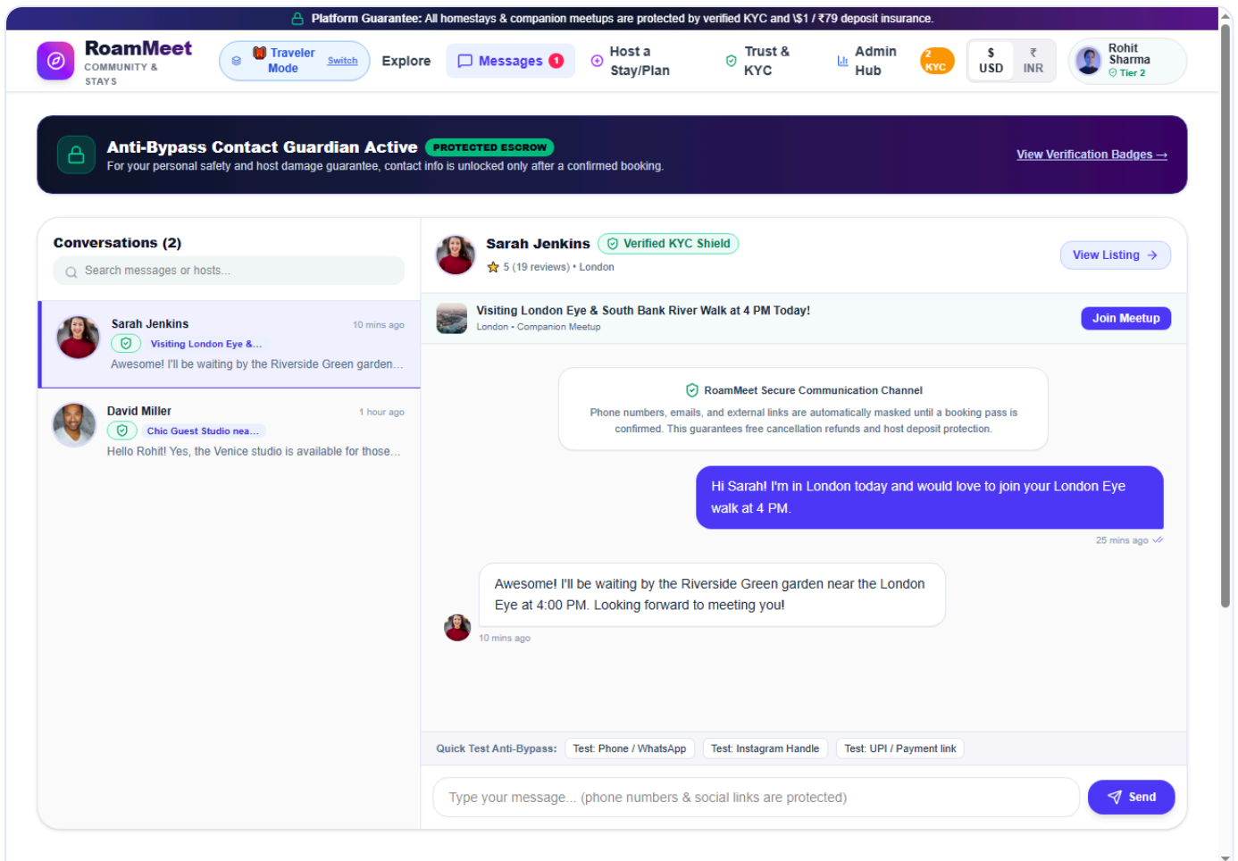
Figure 2: Protected Chat Messenger — Pinned listing header, in-chat booking CTA, and automated contact masking with live typing warning.
