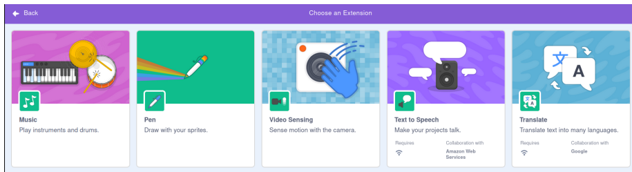
Figure 1: Extensions page
