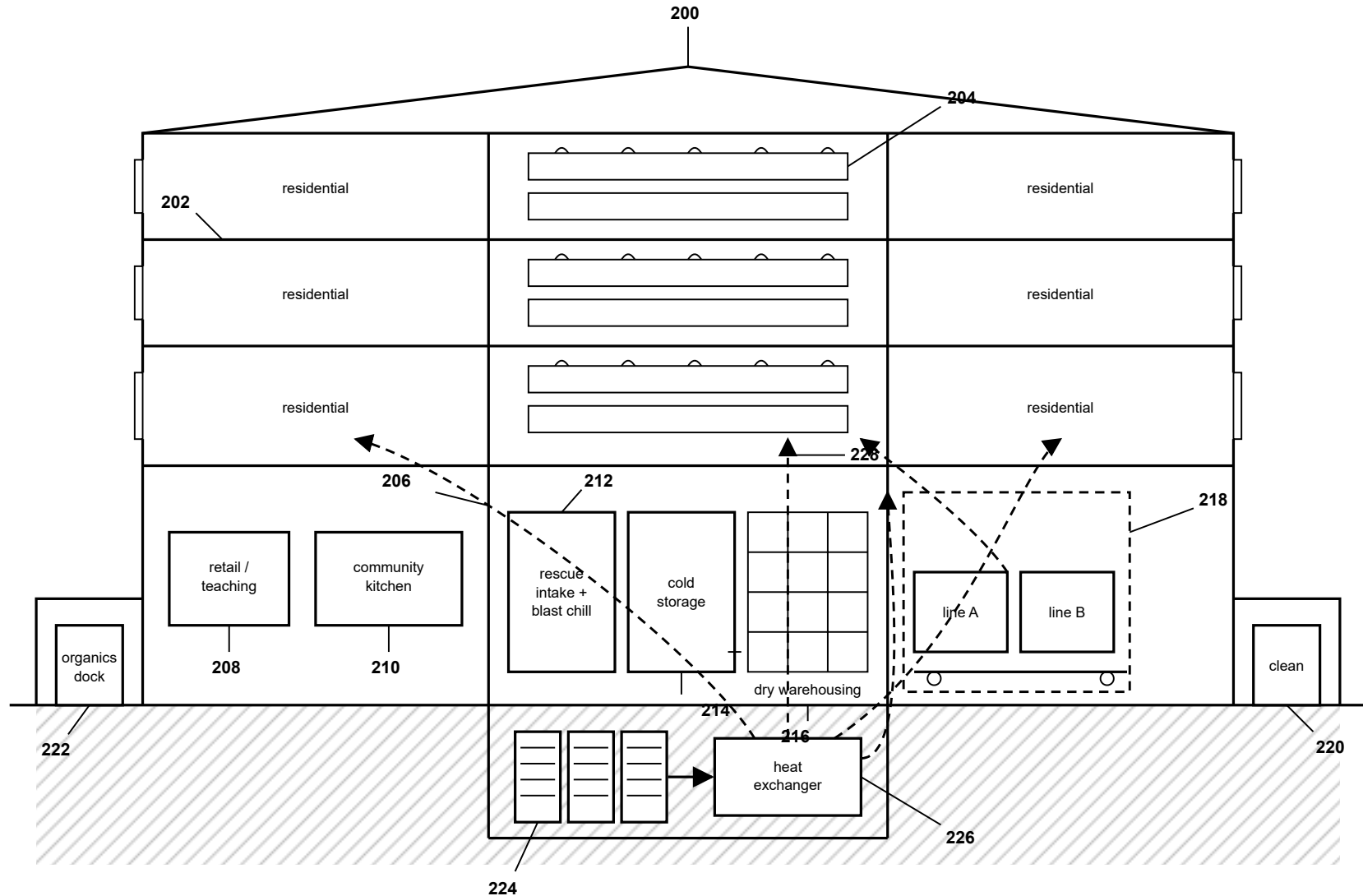
FIG. 2 — Urban Metabolic Hub, Cross-Section (Adaptive Reuse)
