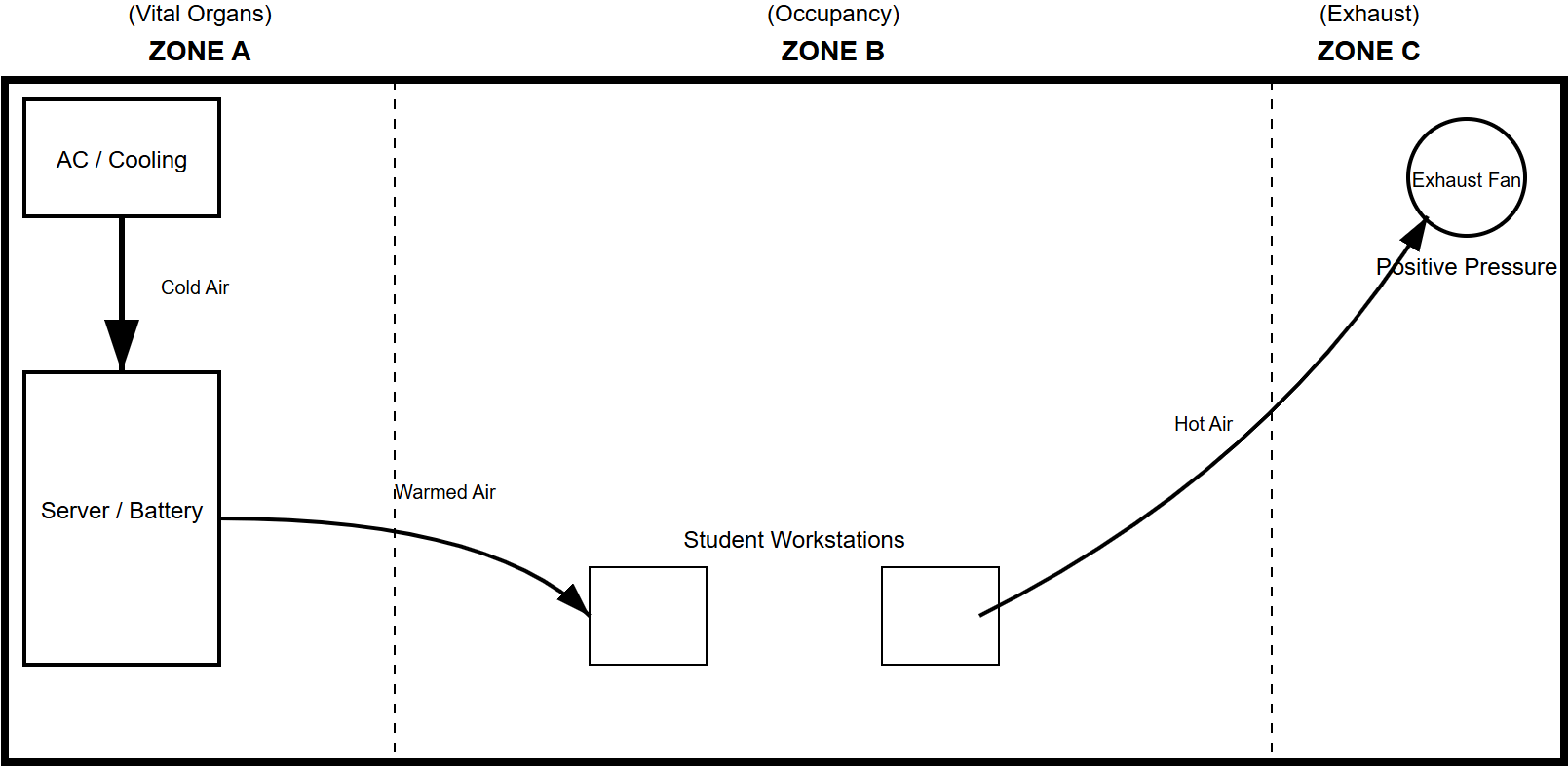
FIG. 3: THERMAL CASCADE TOPOLOGY
