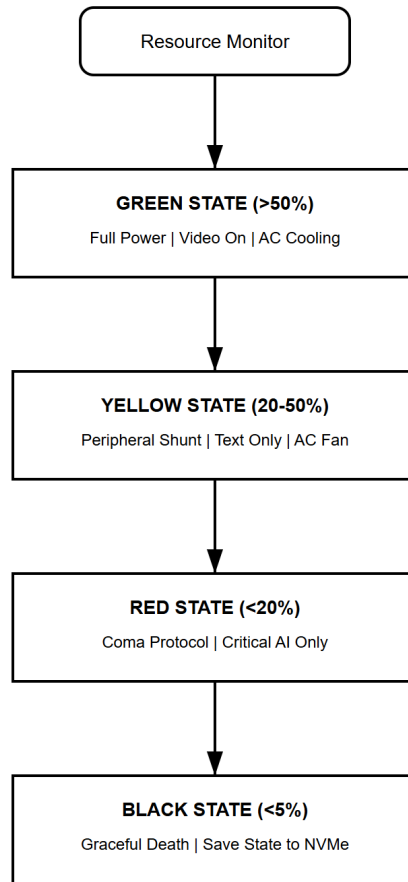
FIG. 2: BIOMIMETIC TRIAGE LOGIC
