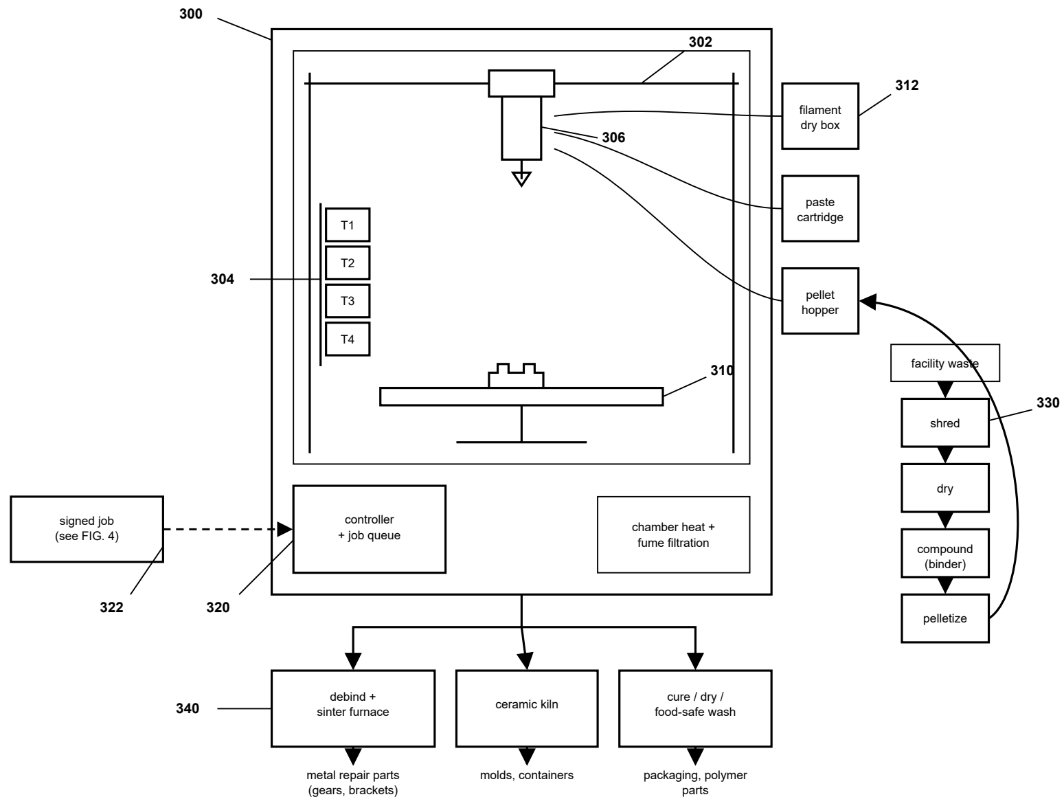
FIG. 3 — Multi-Modal Fabrication Node (one chassis, many material classes)
