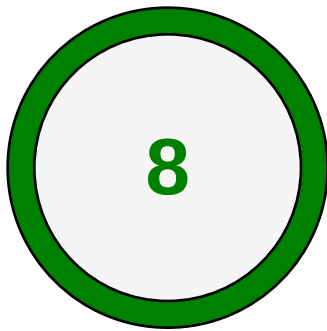
NPA Score
