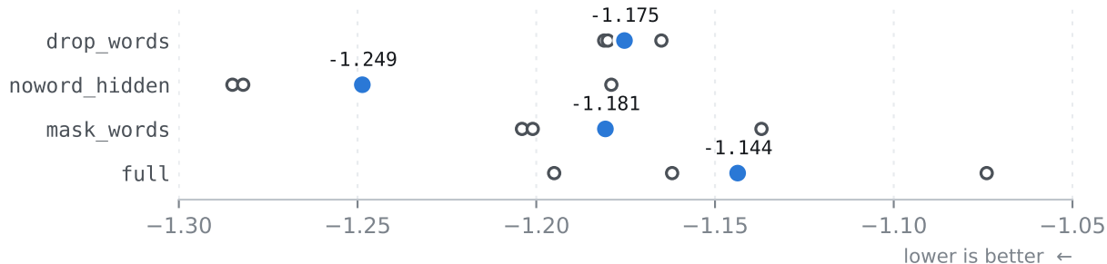
Stroke negative log-likelihood (nats), stroke ladder
