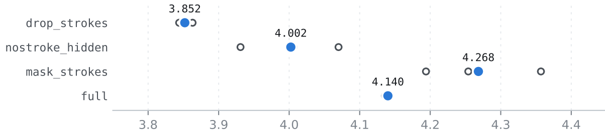
Word cross-entropy (nats), word ladder
