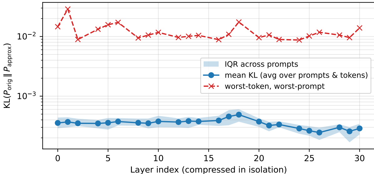
Per-layer KL under rank-16 state compression Qwen/Qwen3.5-4B, 30 prompts
