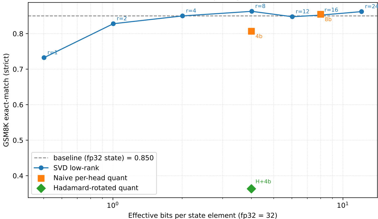
Qwen3.5-4B GSM8K accuracy vs recurrent-state compression (5-shot, 1319 samples, greedy)
