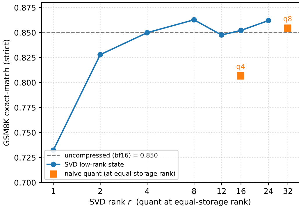
Recurrent-state rank vs. accuracy
