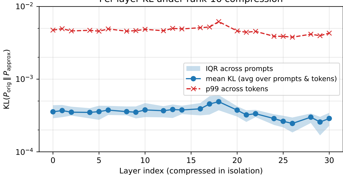
Per-layer KL under rank-16 compression
