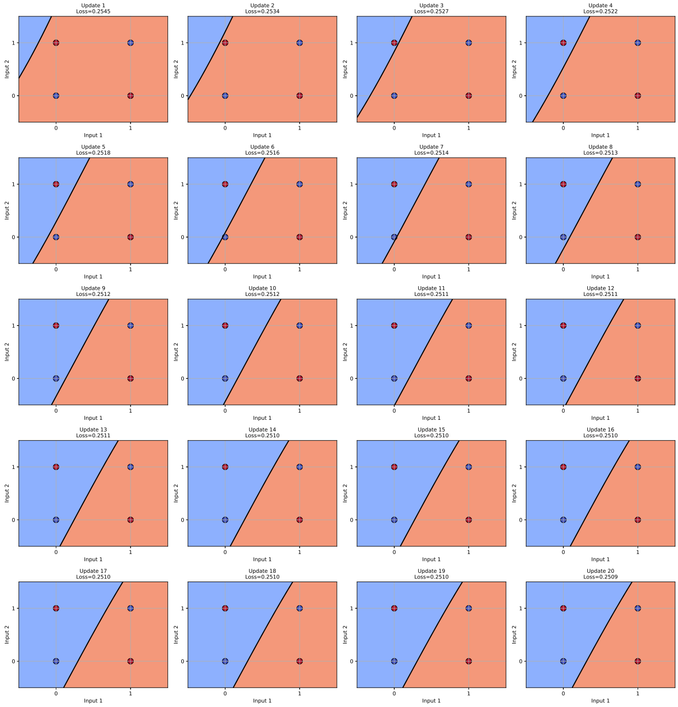
Figure 10: Decision boundary of the XOR gate after each weight update using a Single-Layer Perceptron.
