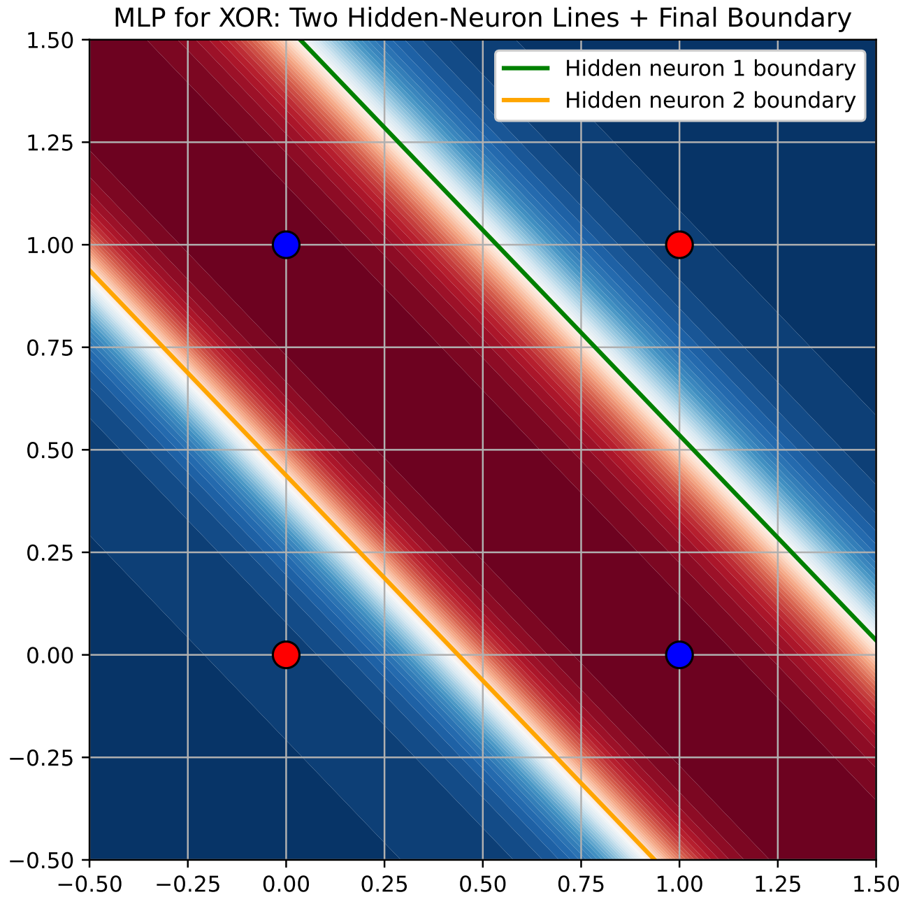
Figure 11: Decision boundary of the XOR gate using a Multi-Layer Perceptron.
