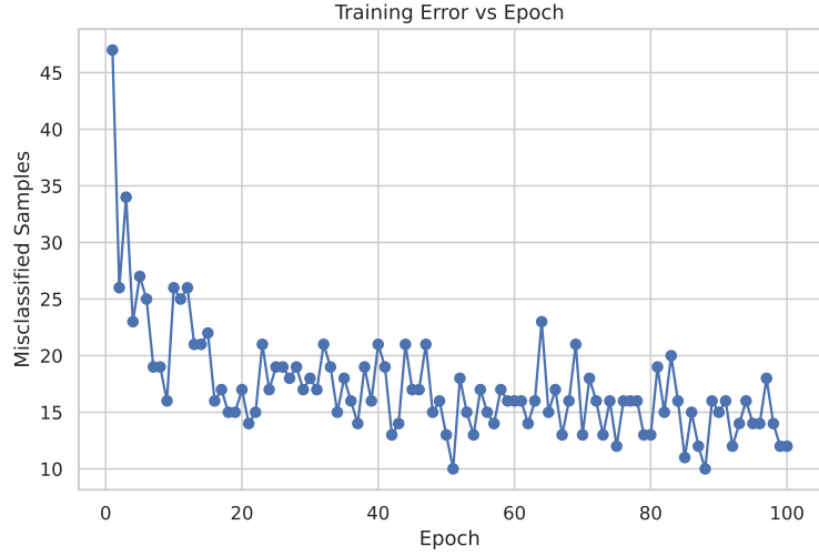
Figure 5: Training Error vs Epoch
