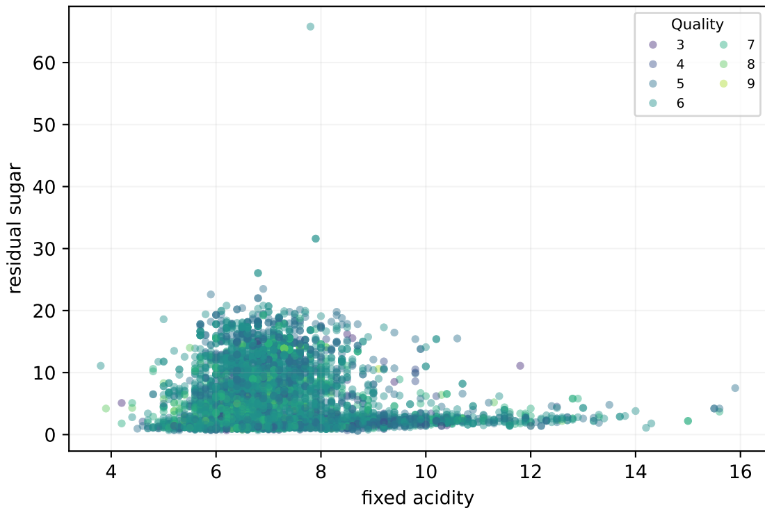
fixed acidity \times residual sugar Pearson \rho = -0.112
