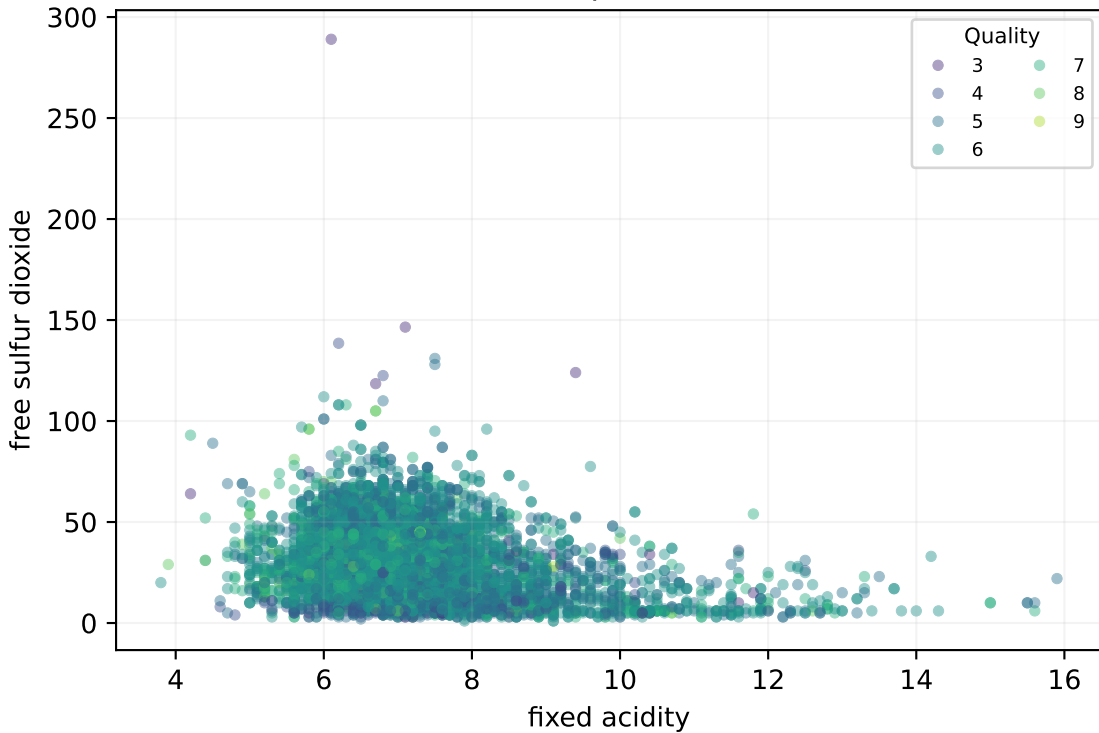
fixed acidity × free sulfur dioxide Pearson \rho = -0.283
