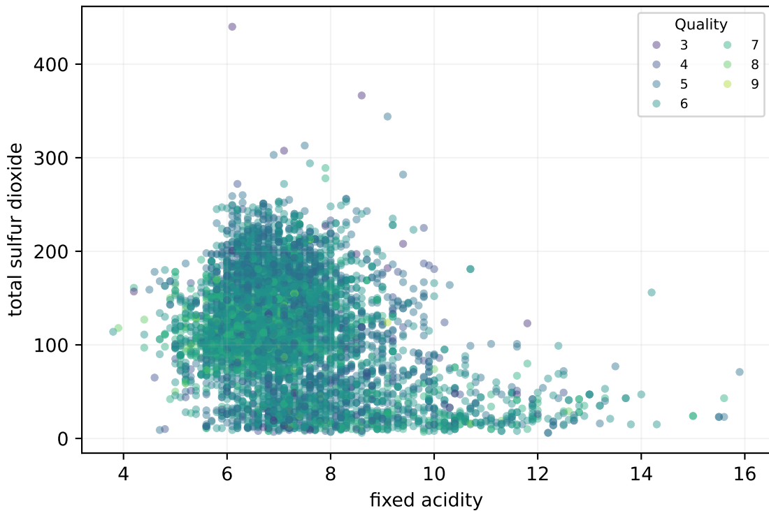
fixed acidity × total sulfur dioxide Pearson \rho = -0.329
