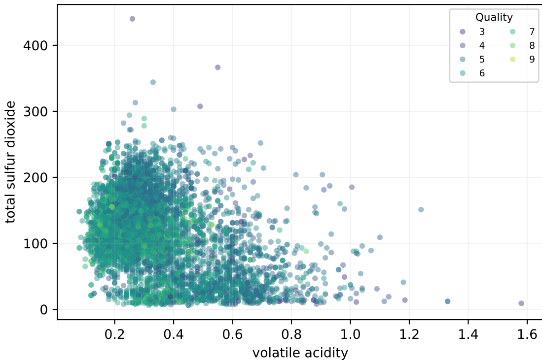
volatile acidity × total sulfur dioxide Pearson \rho = -0.414
