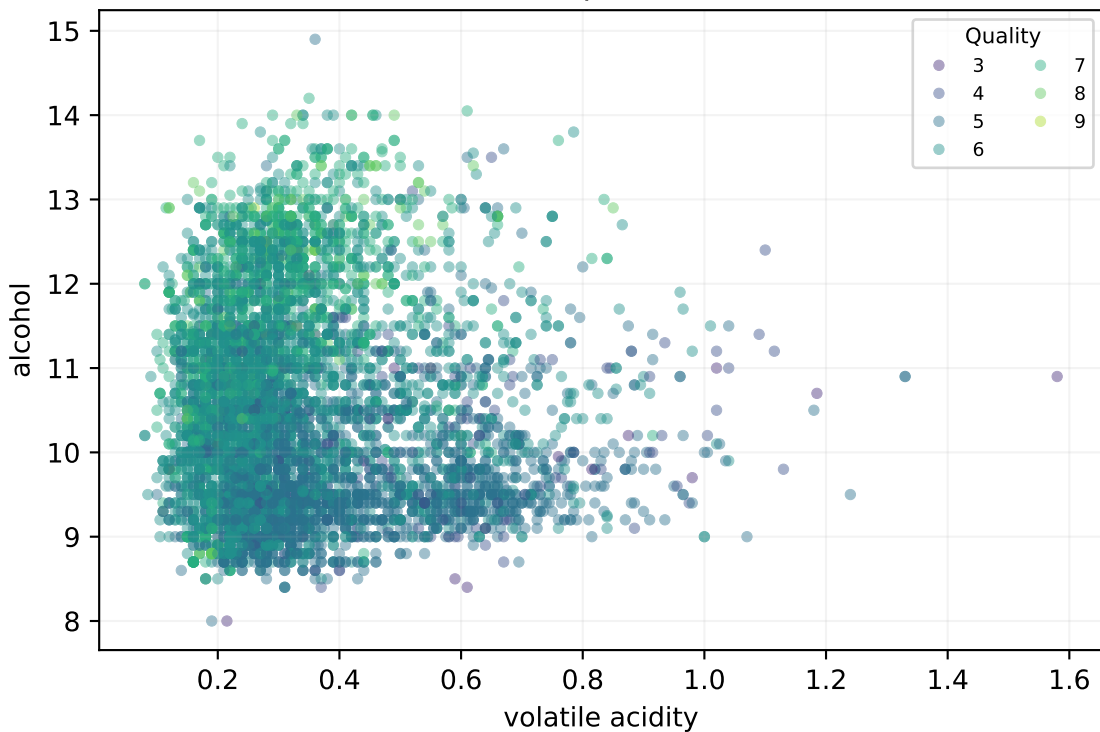
volatile acidity \times alcohol Pearson \rho = -0.038
