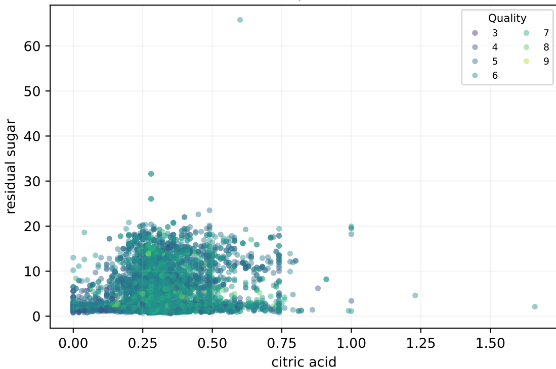
citric acid x residual sugar Pearson \rho = 0.142
