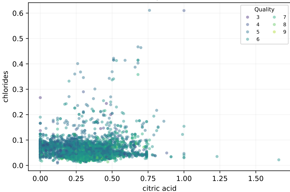
citric acid \times chlorides Pearson \rho = 0.039
