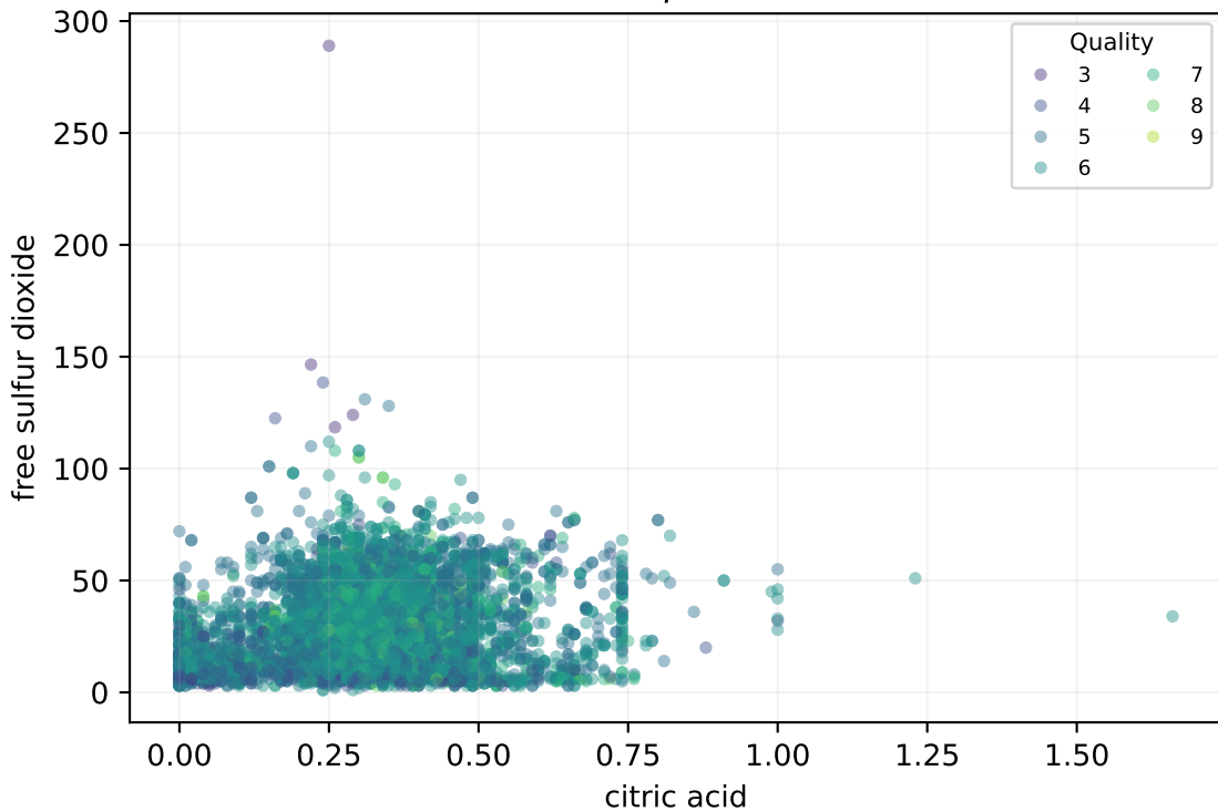
citric acid × free sulfur dioxide Pearson \rho = 0.133
