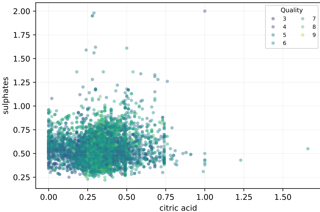
citric acid × sulphates Pearson \rho = 0.056
