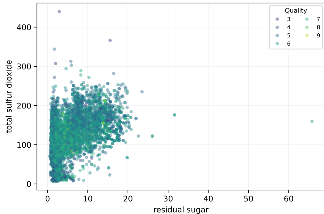
residual sugar \times total sulfur dioxide Pearson \rho = 0.495
