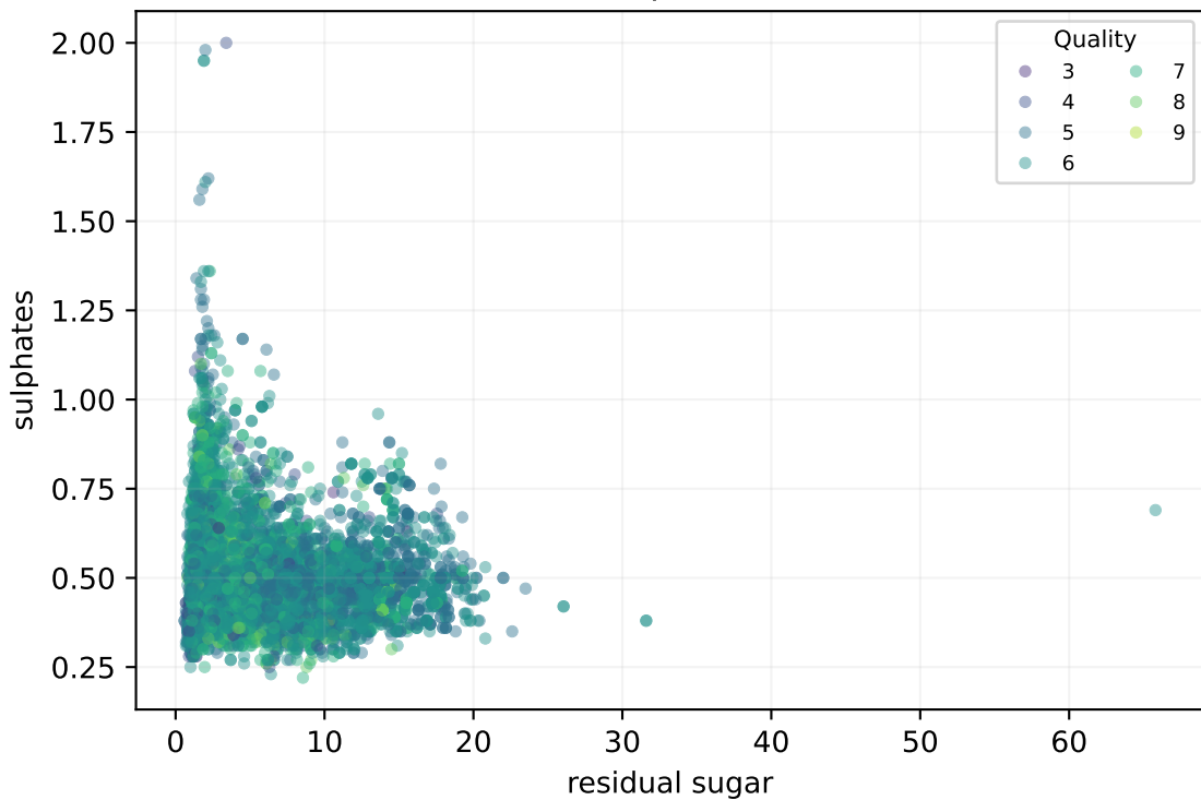
residual sugar \times sulphates Pearson \rho = -0.186
