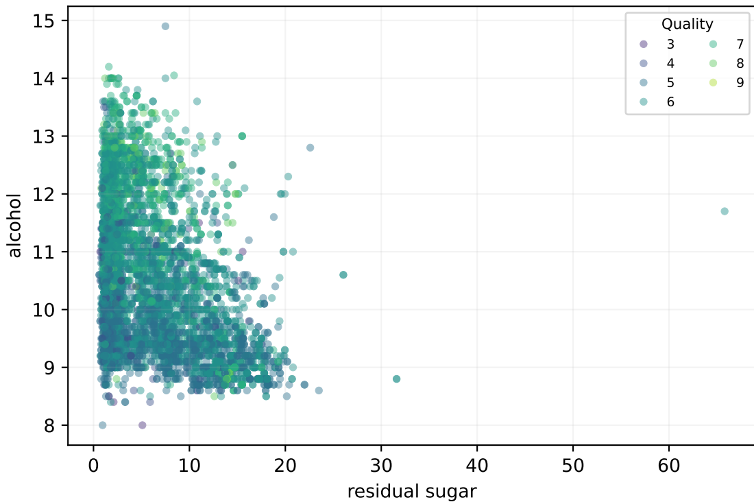
residual sugar \times alcohol Pearson \rho = -0.359
