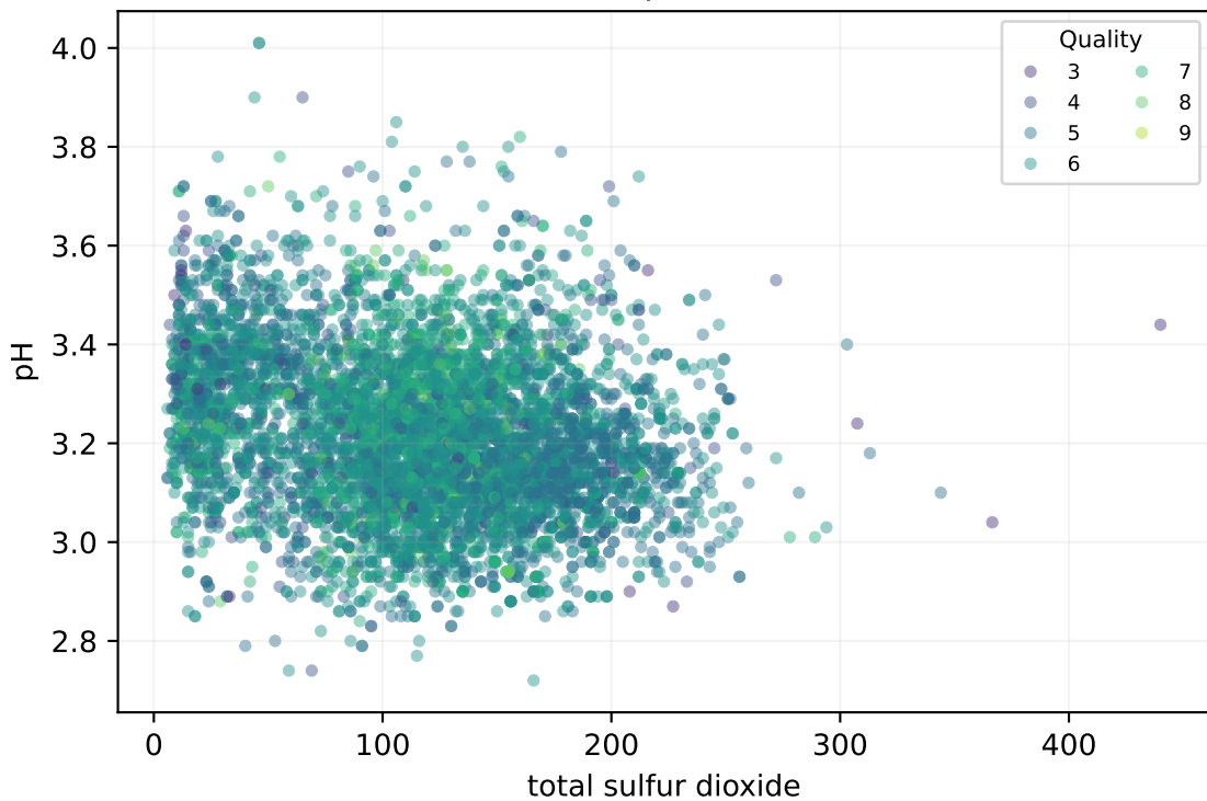
total sulfur dioxide \times pH Pearson \rho = -0.238
