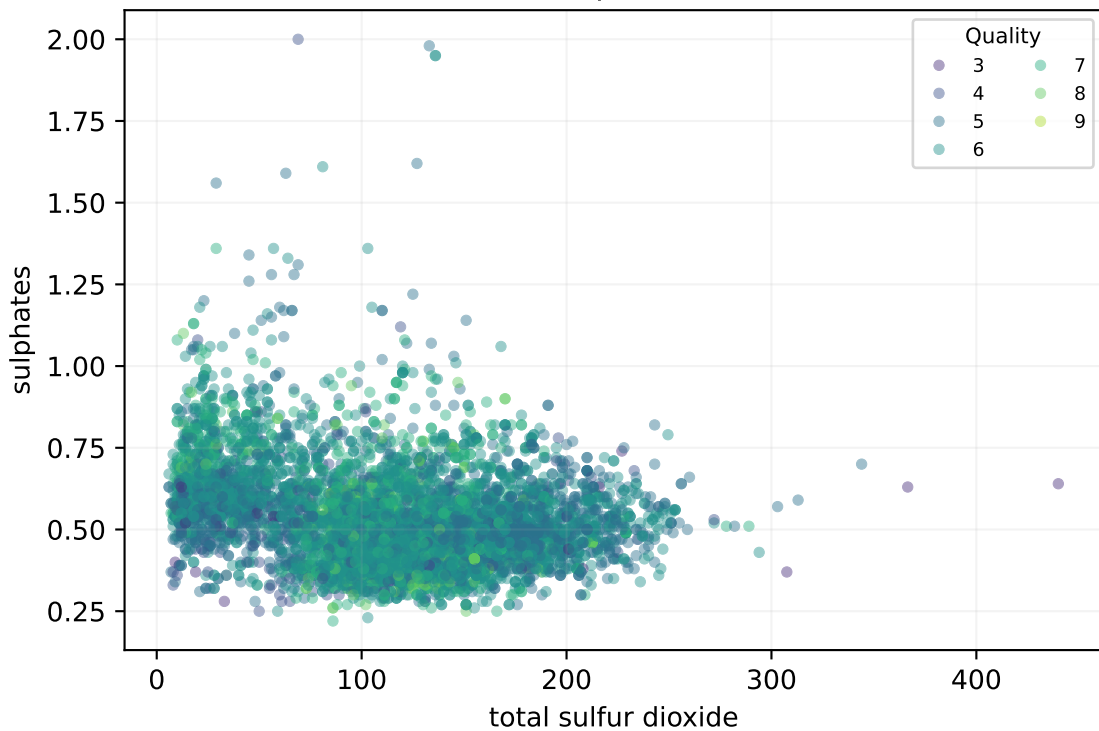
total sulfur dioxide \times sulphates Pearson \rho = -0.276
