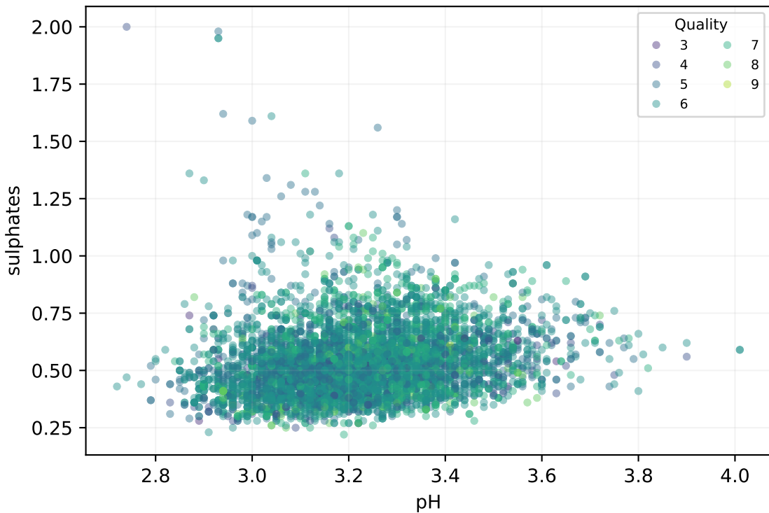
pH × sulphates Pearson \rho = 0.192
