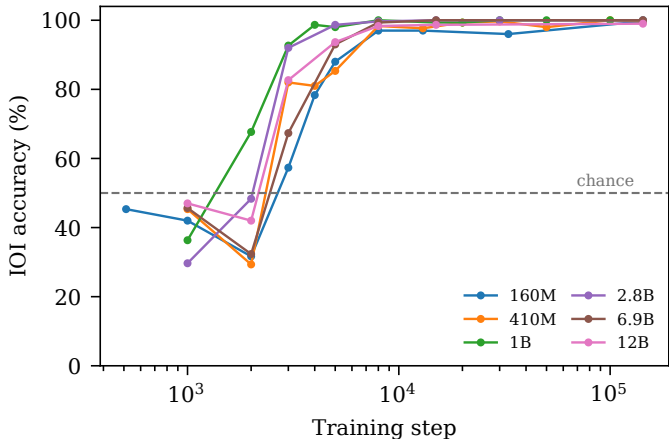
Below-chance window across six scales
