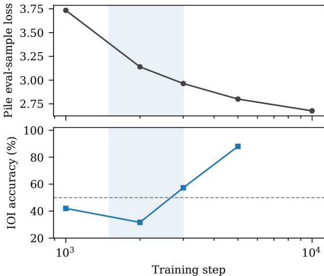
Loss decreases across the sampled checkpoints
