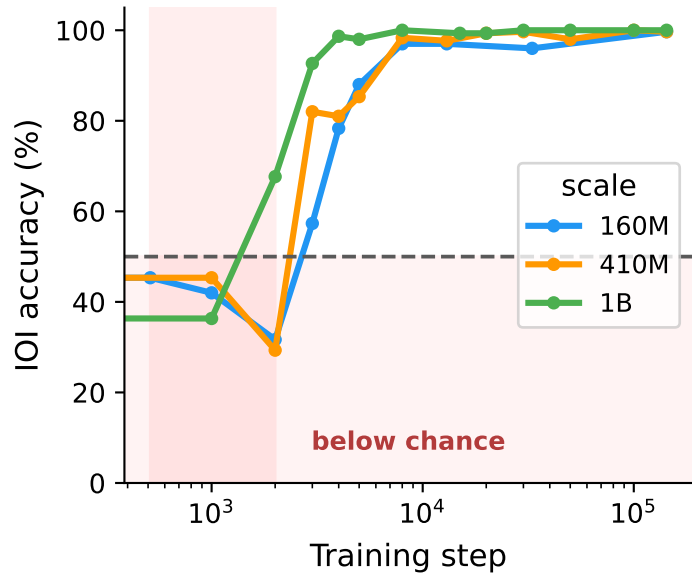
(a) Accuracy dips below chance
