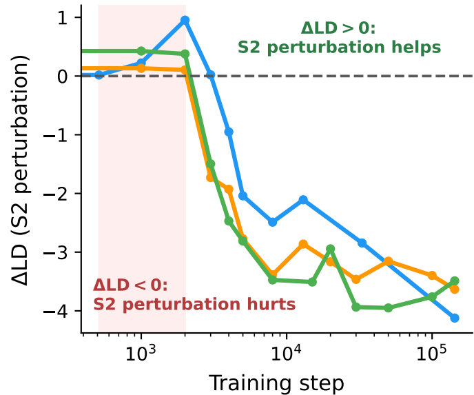
(c) S2 perturbation flips sign
