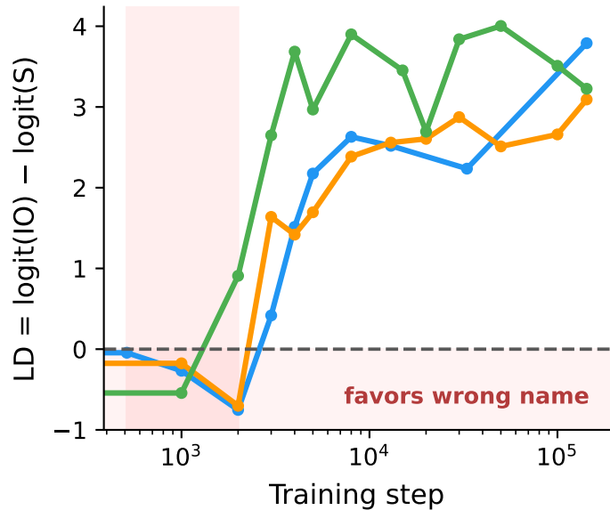
(b) Continuous LD also goes negative
