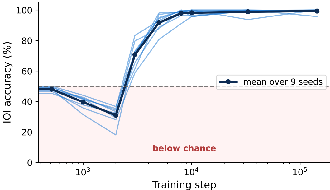
All nine PolyPythias-160M seeds dip below chance
