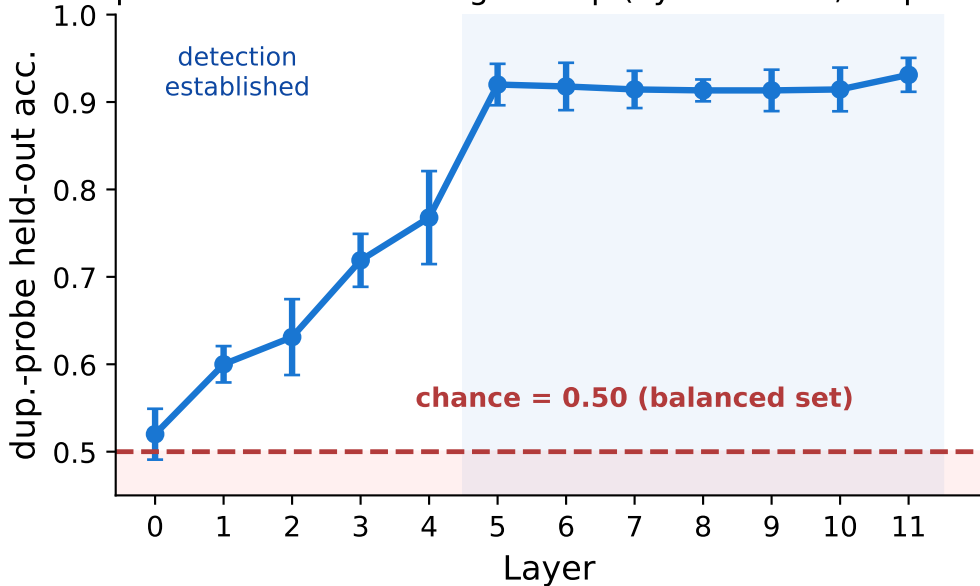
Duplicate detected during the dip (Pythia-160M, step 2000)
