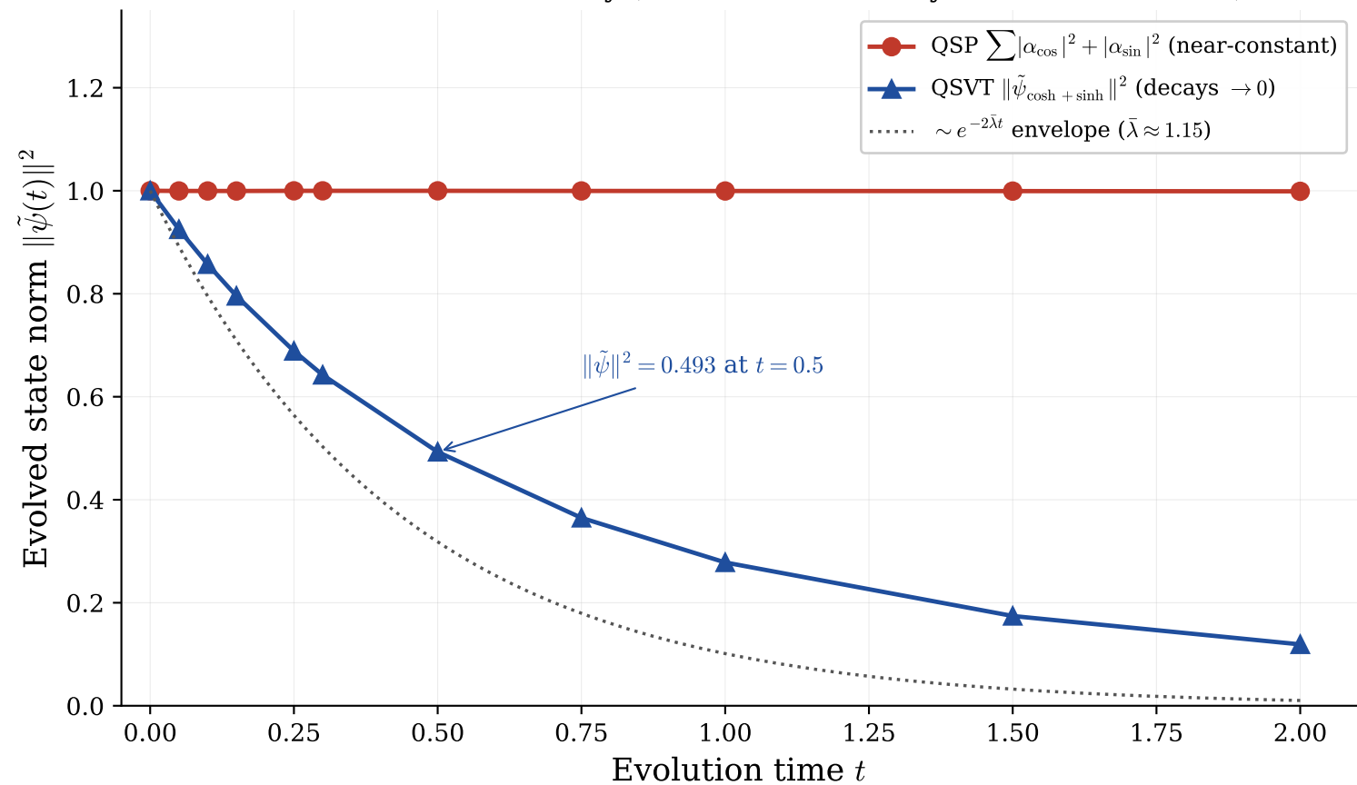
Post-selection norm decay (threshold 0.20, 8-layer AAE, statevector)
