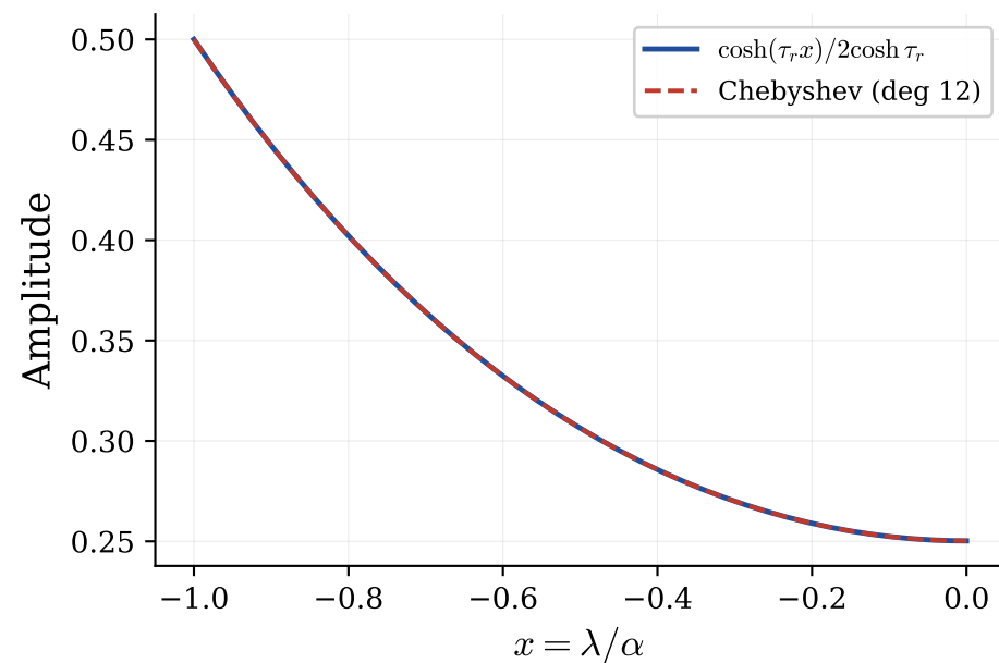
(c) Combined e^{\tau x} reconstruction
